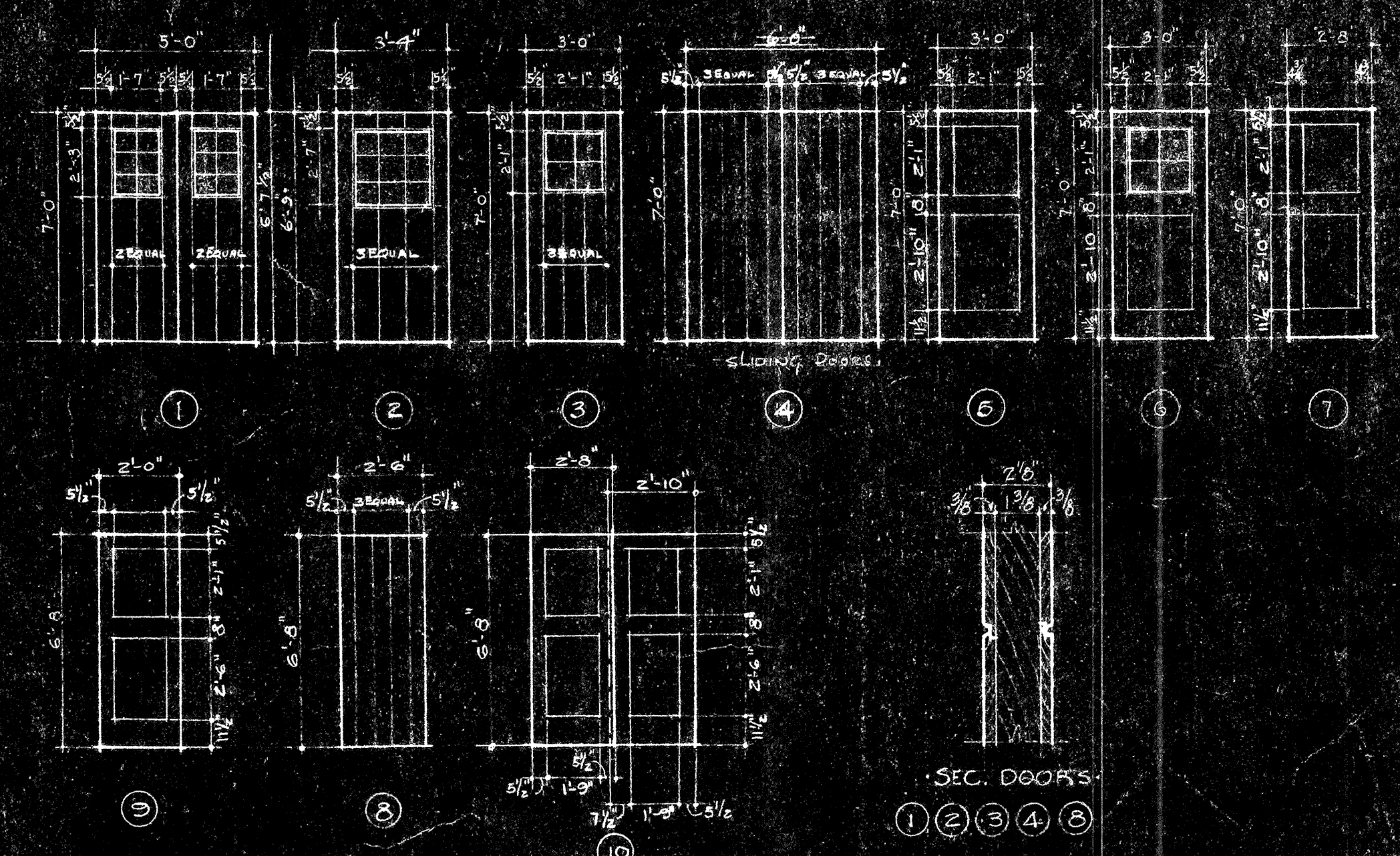
DOOR SCHEDULE SCALE 1/8"=1'-0"
