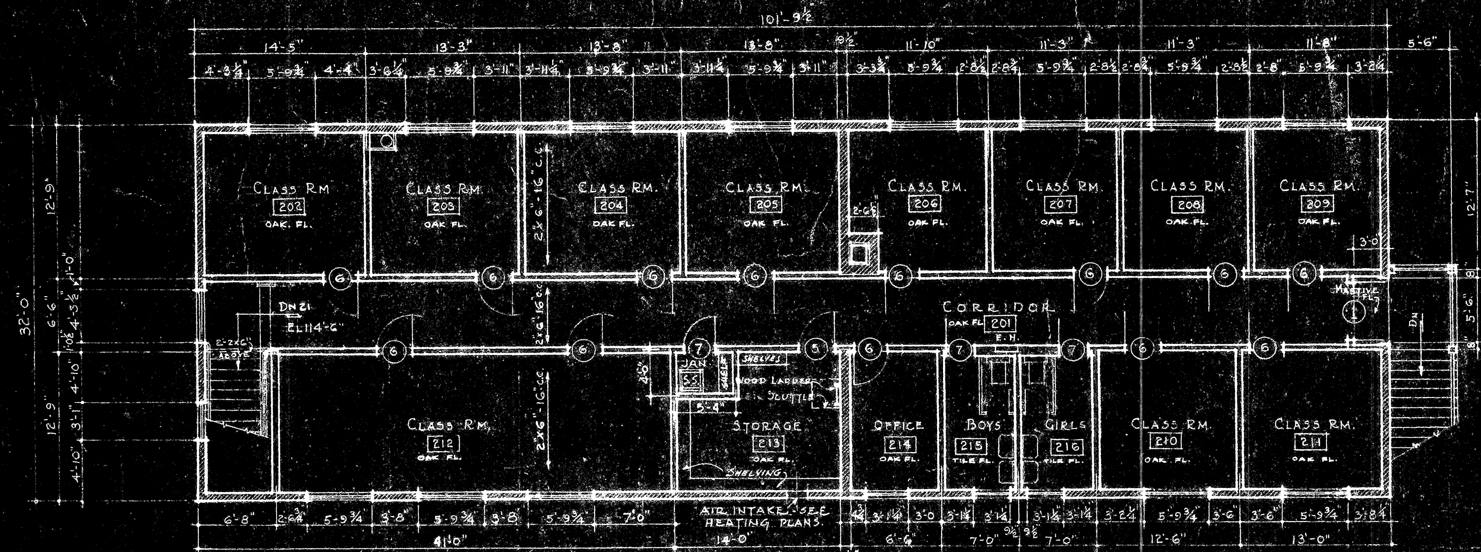
SECOND FLOOR SCALE 1/8"=1'-0"
